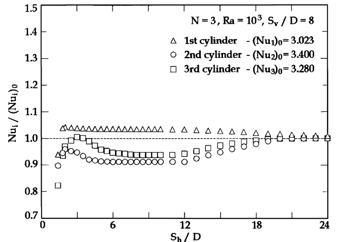
Fig. 13. Distributions of the ratio Nu_i/(Nu_i)_0 vs. S_h/D , for N = 3 , Ra = 10^3 , and S_v/D = 8 .
