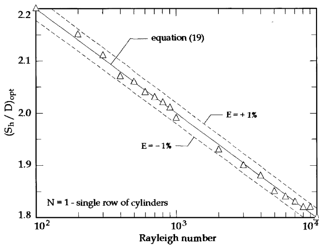
Fig. 7. Distribution of (S_h/D)_{opt} vs. Ra for N = 1 .
