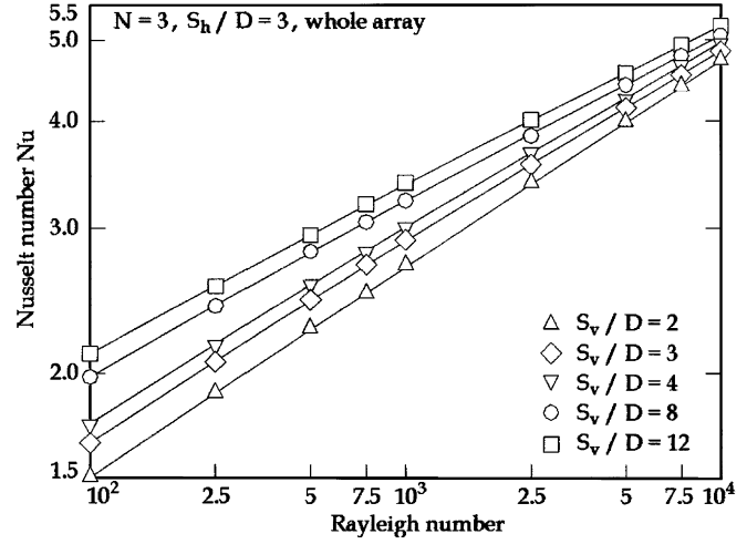
Fig. 21. Distributions of Nu vs. Ra for N = 3 , S_v/D = 3 , and different values of S_h/D .
