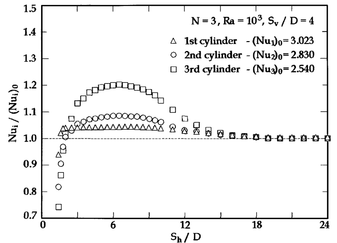
Fig. 12. Distributions of the ratio Nu_i/(Nu_i)_0 vs. S_h/D , for N = 3 , Ra = 10^3 , and S_v/D = 4 .
