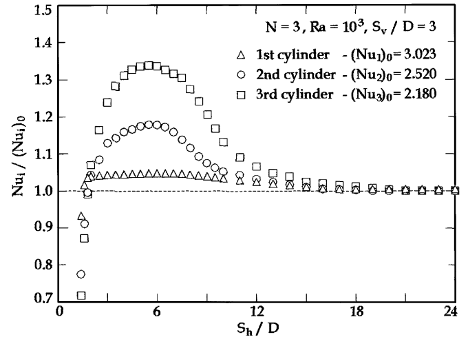
Fig. 11. Distributions of the ratio Nu_i/(Nu_i)_0 vs. S_h/D , for N = 3 , Ra = 10^3 , and S_v/D = 3 .
